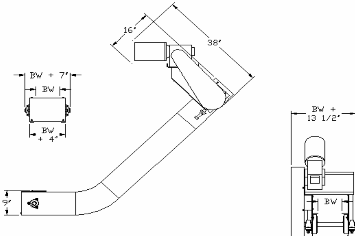
45° TOP MOUNT DRIVE
